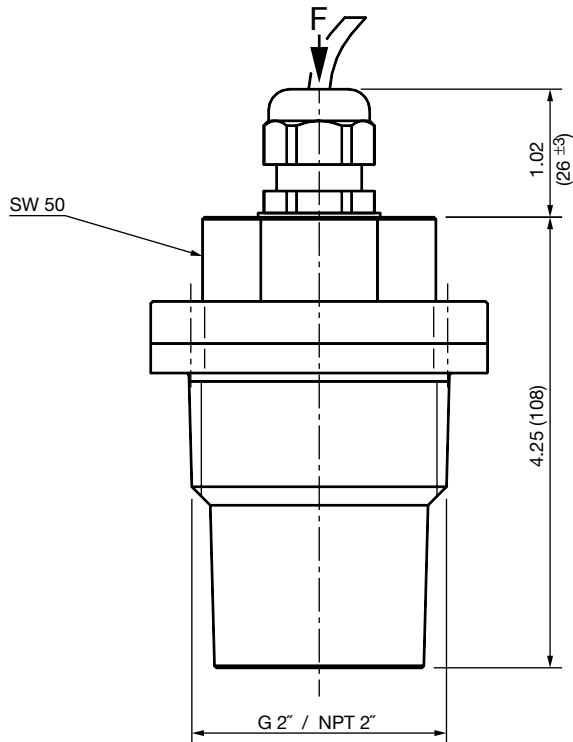
Remote control ultrasonic probe
