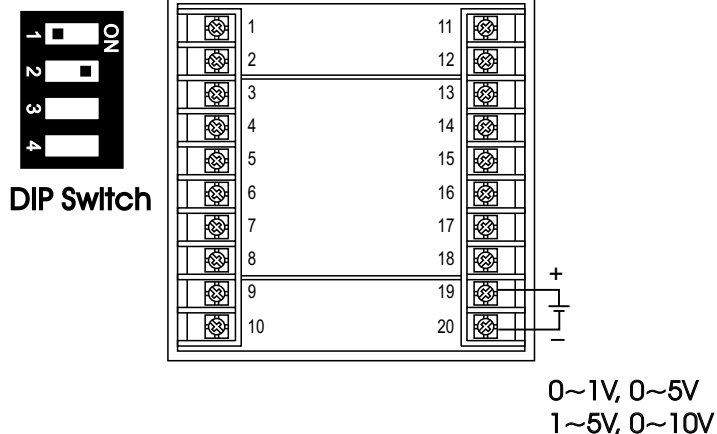
Figure 2.9 Input 2 Linear Voltage Wiring
