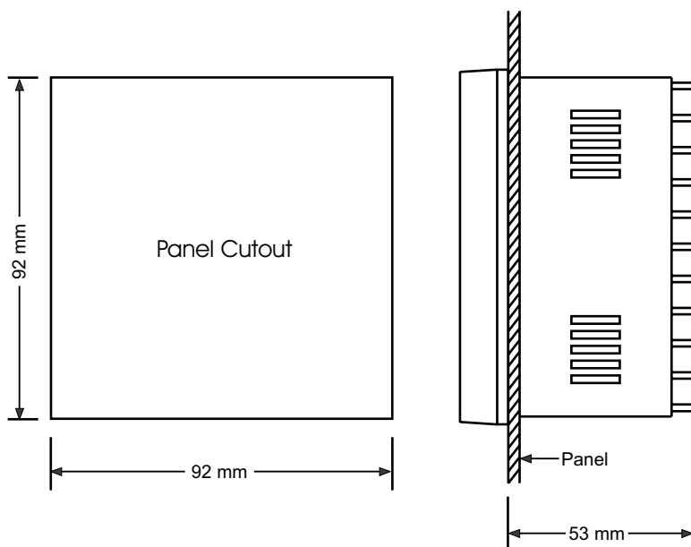
Figure 2.1 Mounting Dimensions
