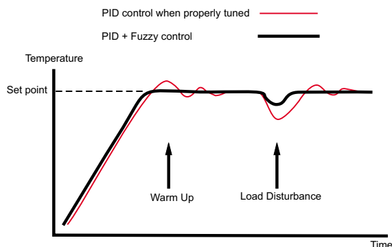
Figure 1.1 Fuzzy PID Enhances Control Stability
