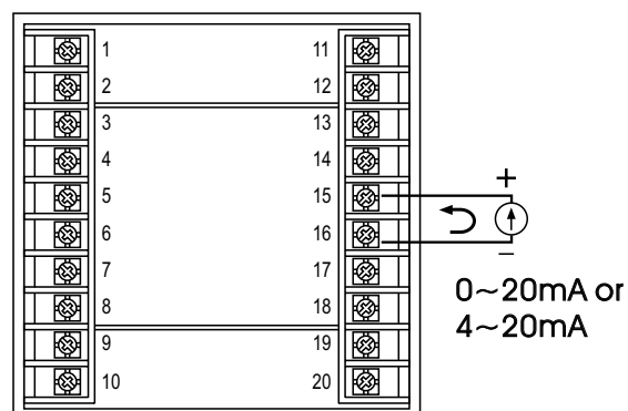
Figure 2.10 Input 2 Linear Current Wiring
