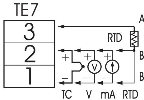
Figure 2.7 Sensor Input Wiring
