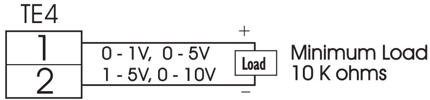
Figure 2.15 Output 2 Linear Voltage
