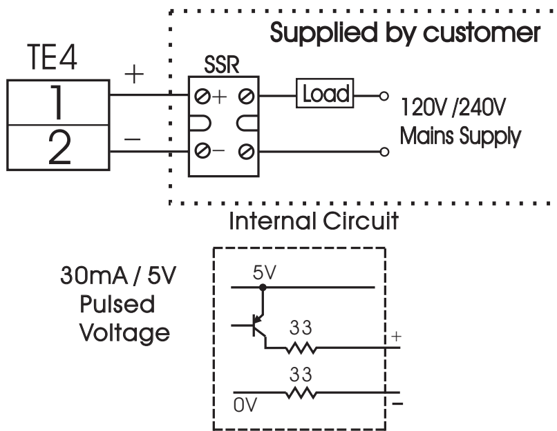
Figure 2.13 Output 2 Pulsed Voltage to Drive SSR
