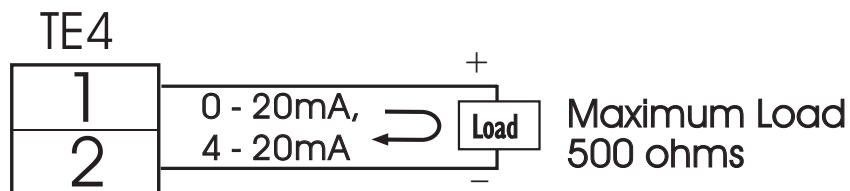
Figure 2.14 Output 2 Linear Current
