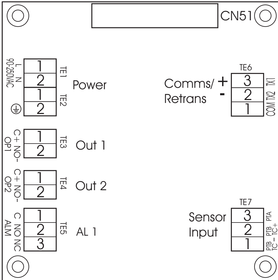
Figure 2.4 Terminal Connection
