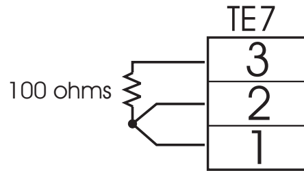
Figure 5.1 RTD Calibration
