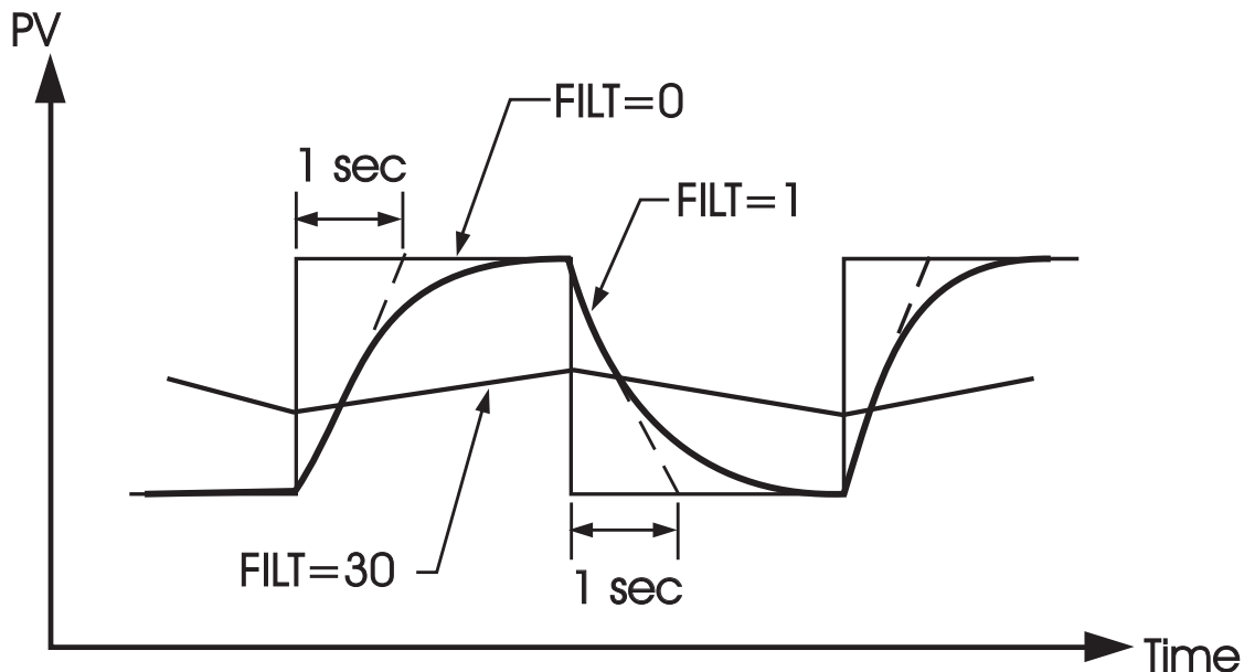
Figure 3.8 Filter Characteristics
