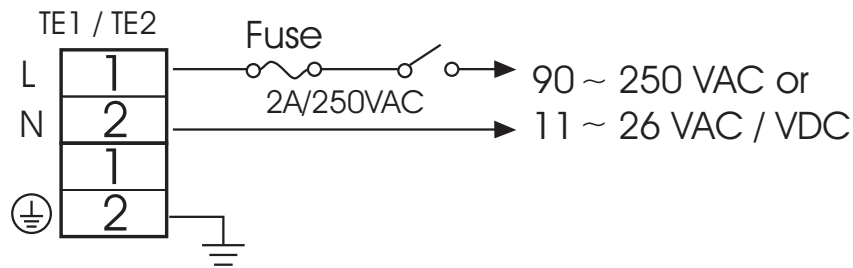
Figure 2.6 Power Supply Connections
