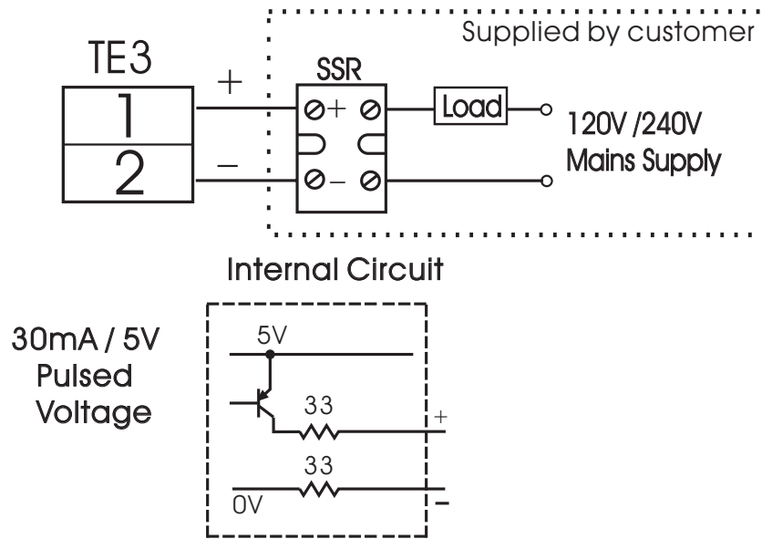
Figure 2.9 Output 1 Pulsed +5 VDC Voltage to Drive SSR
