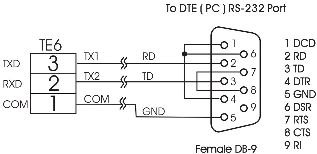
Figure 2.20 Configuration of RS-232 Cable
