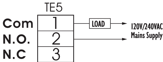
Figure 2.16 Alarm Output to Drive Load
