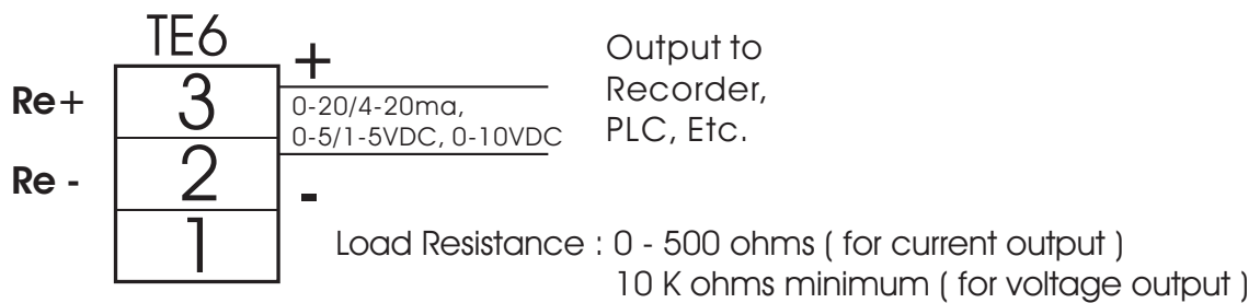
Figure 2.17 Retransmission Output Wiring
