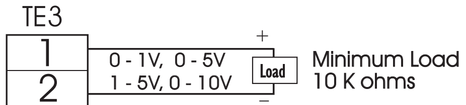
Figure 2.11 Output 1 Linear Voltage
