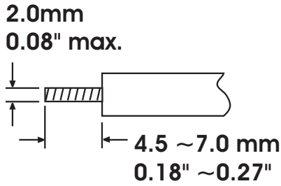
Figure 2.3 Lead Termination
