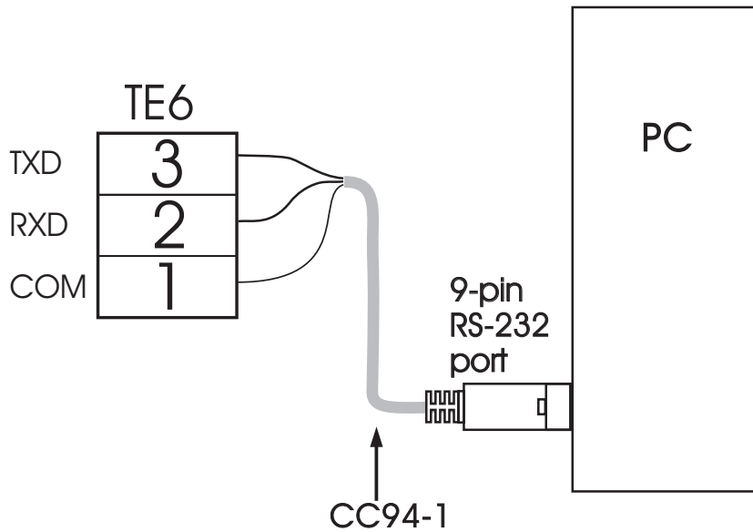
Figure 2.19 RS-232 Wiring
