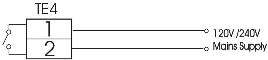
Figure 2.12 Output 2 Relay or Triac (SSR) to Drive Contactor
