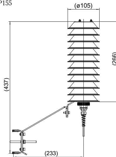
DTR503A pole mast installation.
