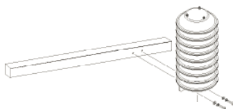
DTR502B horizontal beam installation.
