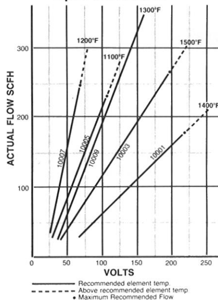
Open Air Heaters
