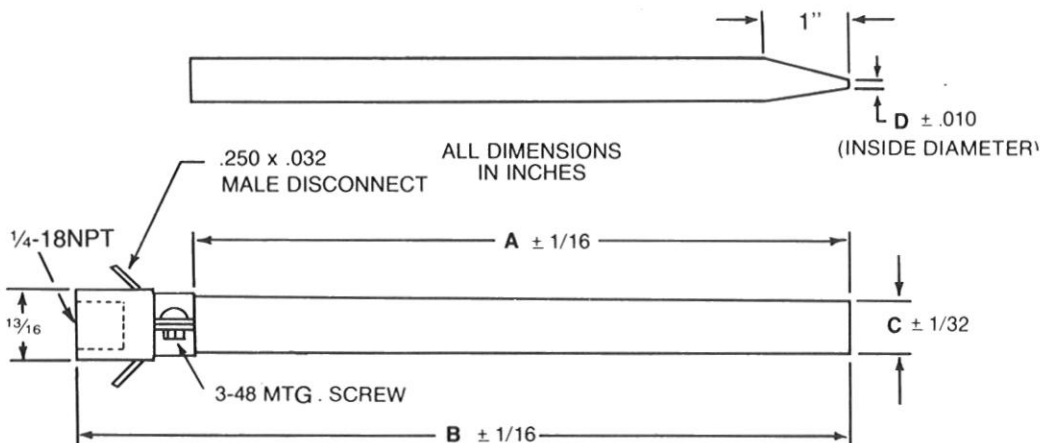
Open Air Heaters
