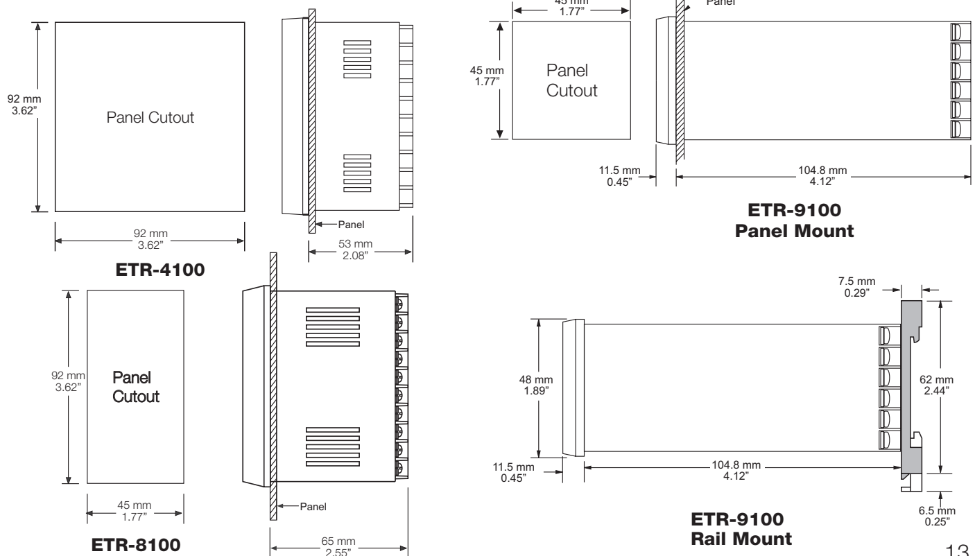
Figure 2.1 Mounting Dimensions
