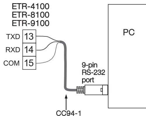
Figure 2.22 RS-232 Wiring
