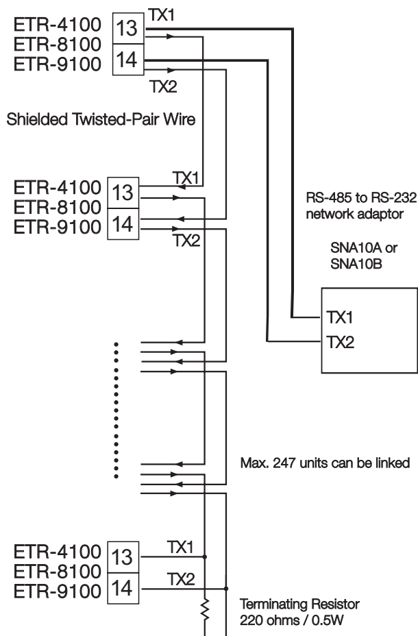
Figure 2.21 RS-485 Wiring
