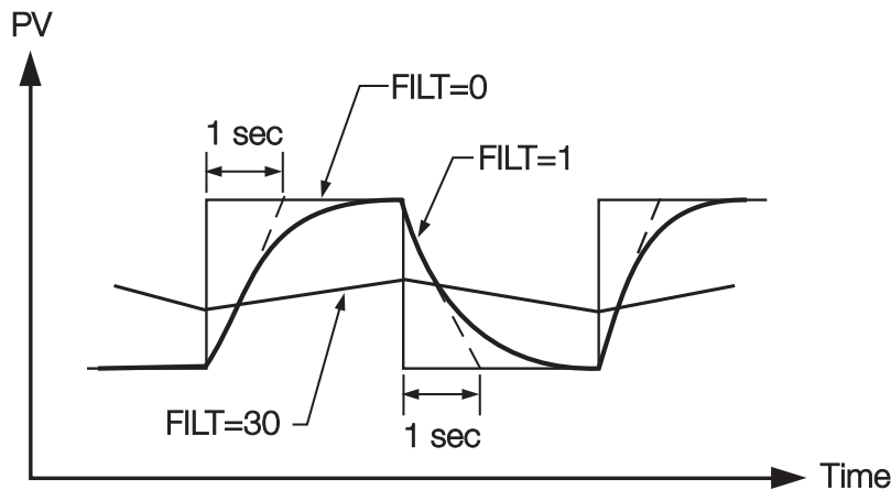
Figure 3.8 Filter Characteristics
