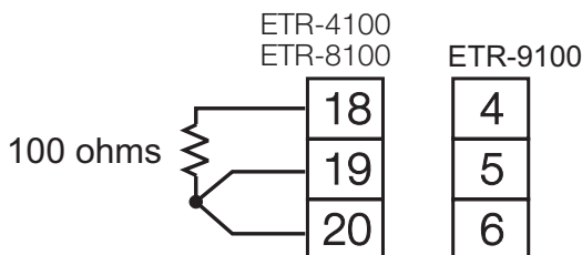
Figure 5.1 RTD Calibration
