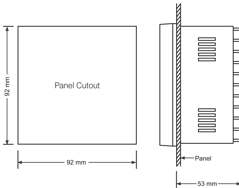
Figure 2.1 Mounting Dimensions
