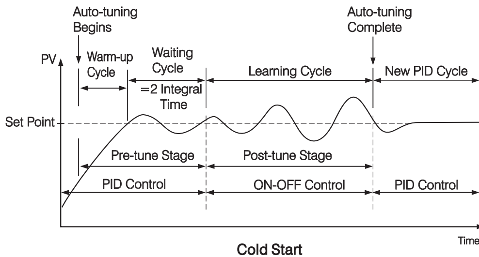
Figure 3.22 Auto-tuning Procedure
