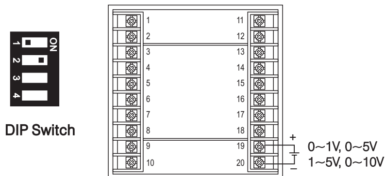
Figure 2.7 Input 1 Linear Voltage Wiring
