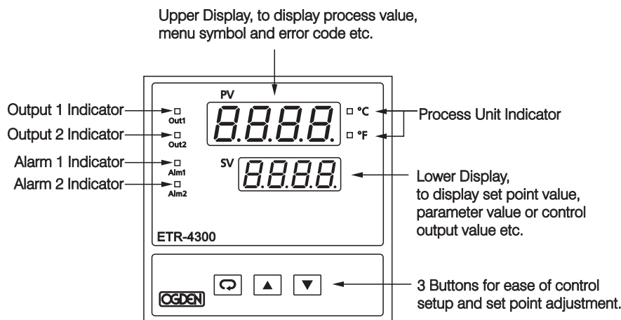
Figure 1.4 Front Panel Description
