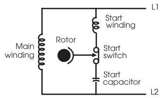
Cap start circuit diagram
